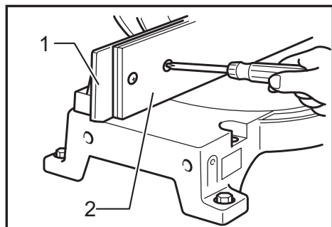
► 1. Guide fence 2. Wood facing
